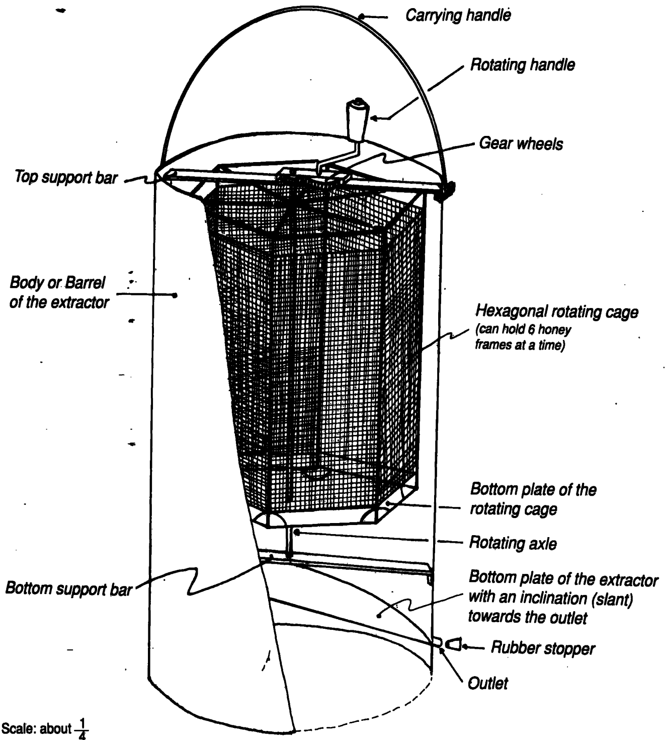
Figure 9.5: Details of a suitable portable honey extractor that is capable of holding 6 honey frames at a time. The handle help in its portability and such an extractor can be very handy.
