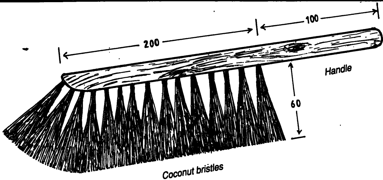
Figure 6.16: A Bee Brush (Not to scale, all dimensions in millimetres).
