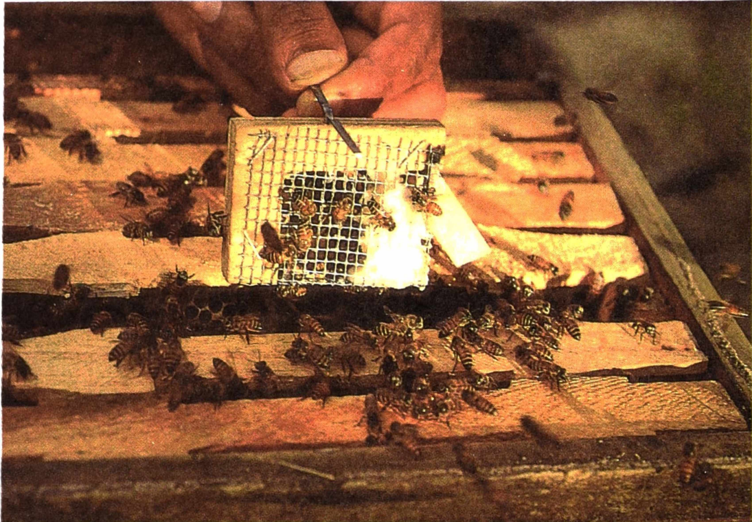
Figure 7.4: Queen cage with queen inside. The entrance plugged with candy paste before opening the door. The cage is about to be inserted between two top-bars. The wire on top now swung out helps to suspend the queen cage between two top bars.
